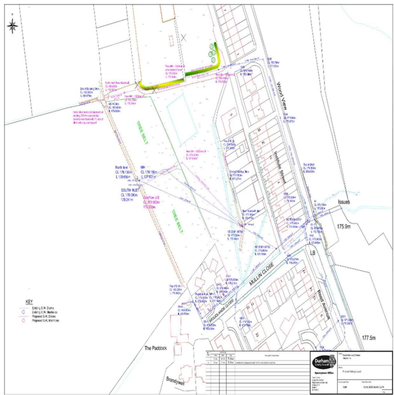
FIGURE 3 PLAN OF FLOOD RISK MITIGATION STRATEGY
